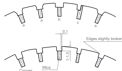
Figure 2: Here it is clear how it should be milled; a bevel is not necessary in most cases, if the collector is turned precisely.
