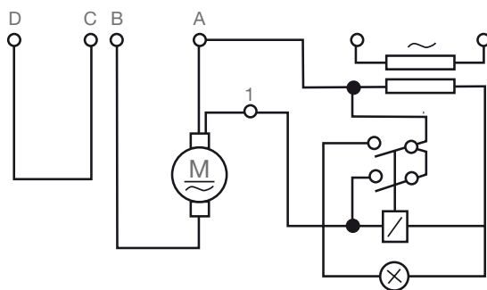
Circuit for signalling device with auxiliary circuit
