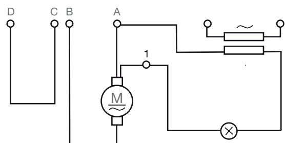
Circuit for signalling device without auxiliary circuit
